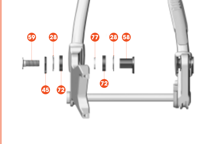
DETAIL 2
